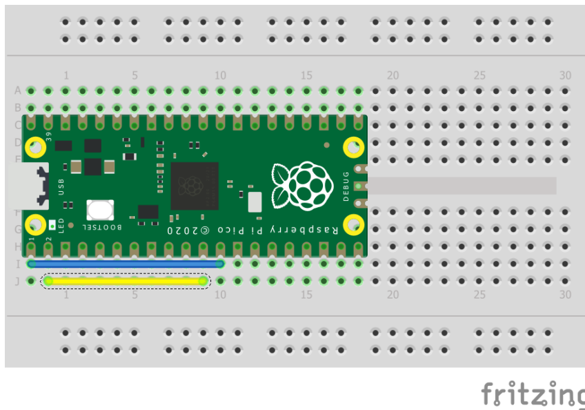
Figure 9. Wiring two of the Pico's ports together. Be sure to wire UART0n TX to UART1 RX and UART0 RX to UART1 TX.
